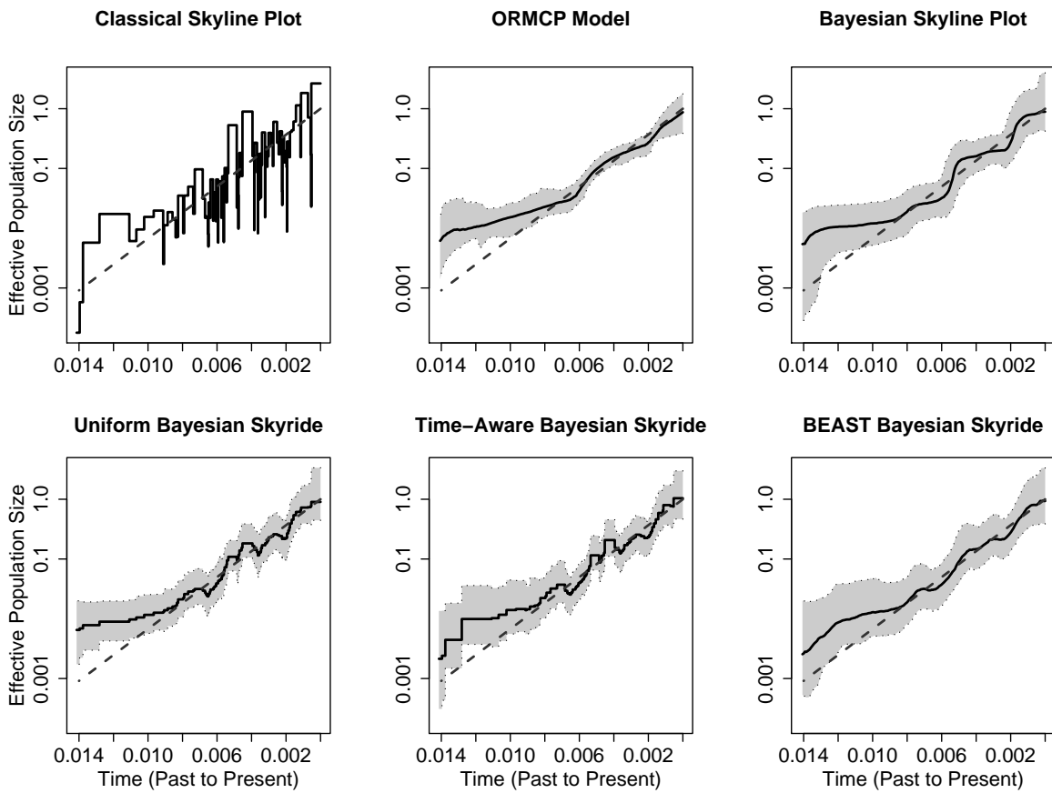
Figure 3: Exponential growth simulation. See Figure 2 for the legend explanation.
