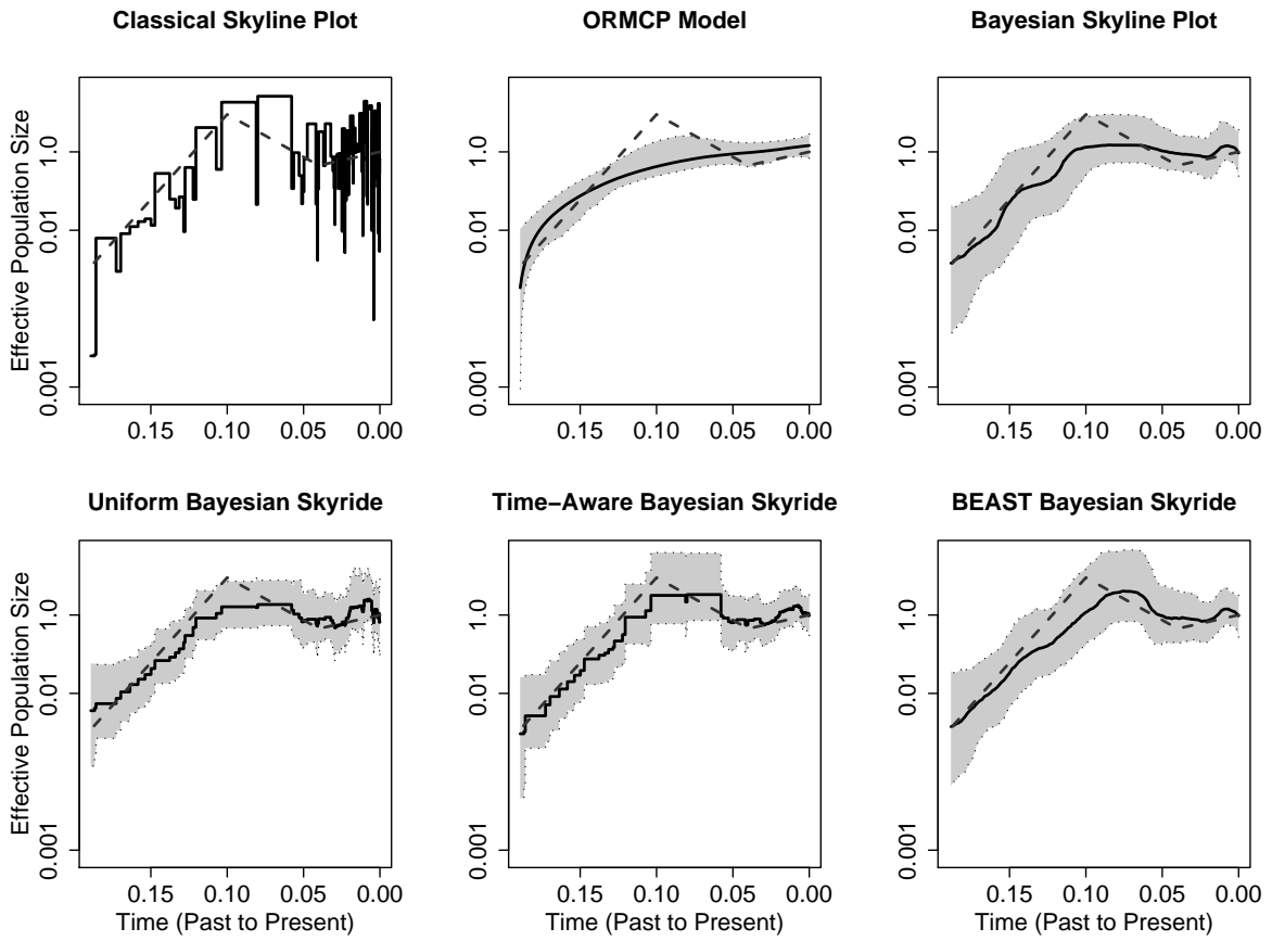
Figure 4: Simulated bottleneck. See Figure 2 for the legend explanation.
