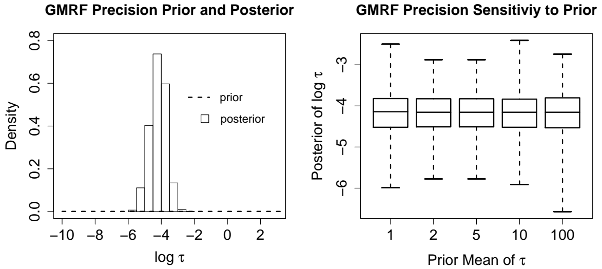
Figure 7: Prior sensitivity. In the left plot, we depict the prior density (dashed line) and posterior histogram (vertical bars) of the log-transformed GMRF precision \tau . The right plot demonstrates five box-plots of the posterior distributions of \log \tau corresponding to five different prior means of \tau . In both plots, we use the Egyptian hepatitis virus C data.
