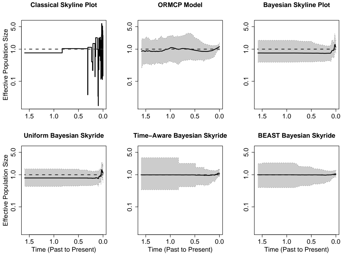
Figure 2: Constant population size simulation. We present a classical skyline plot (solid black line) in the top left part of the figure. The other five plots show posterior median (solid black line) and 95% BCIs (grey shading) of the effective population size under the Opgen-Rhein multiple change-point (ORMCP) model, Bayesian skyline plot, time-aware and uniform Bayesian skyrides with a fixed genealogy, and BEAST Bayesian skyride method. In all six plots, the dashed lines represent the “true” population size trajectory that was used for simulations. Here and in all subsequent plots of effective population sizes, we use the log transformation of the population size-axis.
