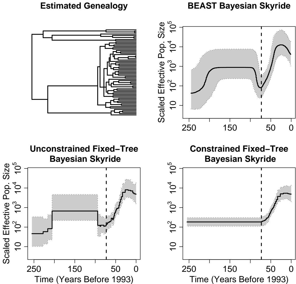
Figure 5: Egyptian hepatitis C virus (HCV). In the top left corner, we show the estimated genealogy of the HCV sequences. The rest of the plots demonstrate posterior medians (solid lines) and 95% BCIs (shaded grey areas) of the scaled effective population size trajectories under the BEAST Bayesian skyride (top right), unconstrained (bottom left), and constrained (bottom right) fixed-tree time-aware Bayesian skyride analyses. In the constrained model the effective population size is forced to be constant prior to the 1920s.
